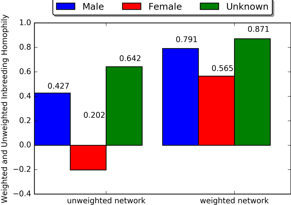
Homophily by gender in Github Followers Network Homophily by gender in Github Accapcted Pull Request Network
