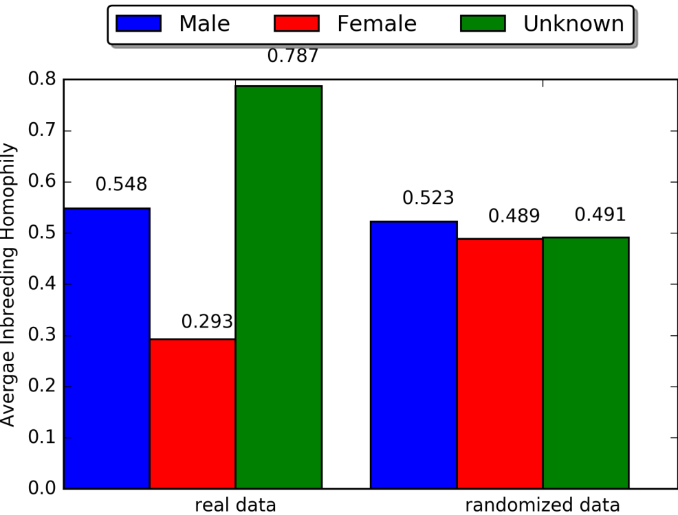
Homophily by gender in Github Followers Network Homophily by gender in Github Accapcted Pull Request Network
